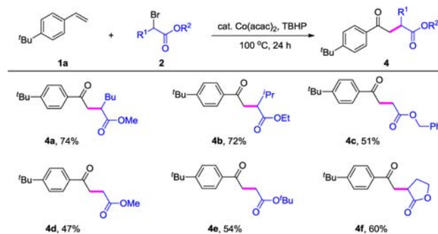
Scheme 3. Scope of \alpha -Bromoesters a
