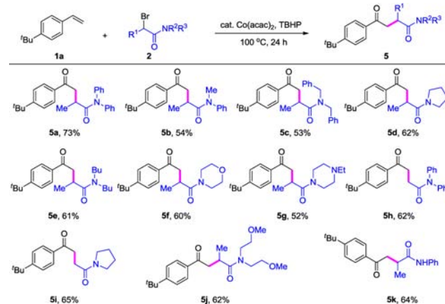
Scheme 4. Scope of \alpha -Bromoamides a
