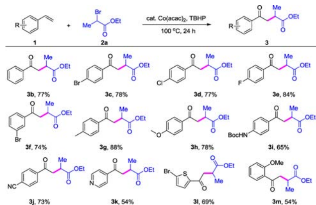
Scheme 2. Scope of Styrenes a
